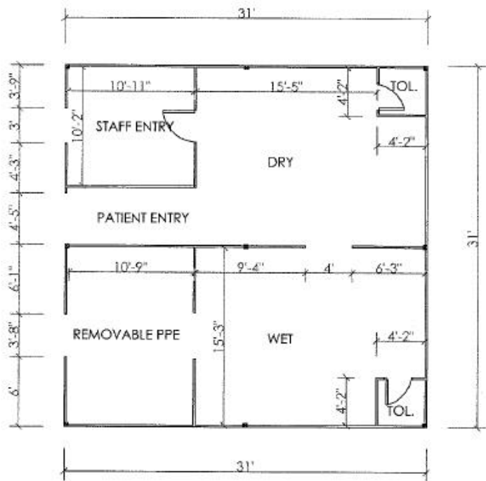
FLOOR PLAN
